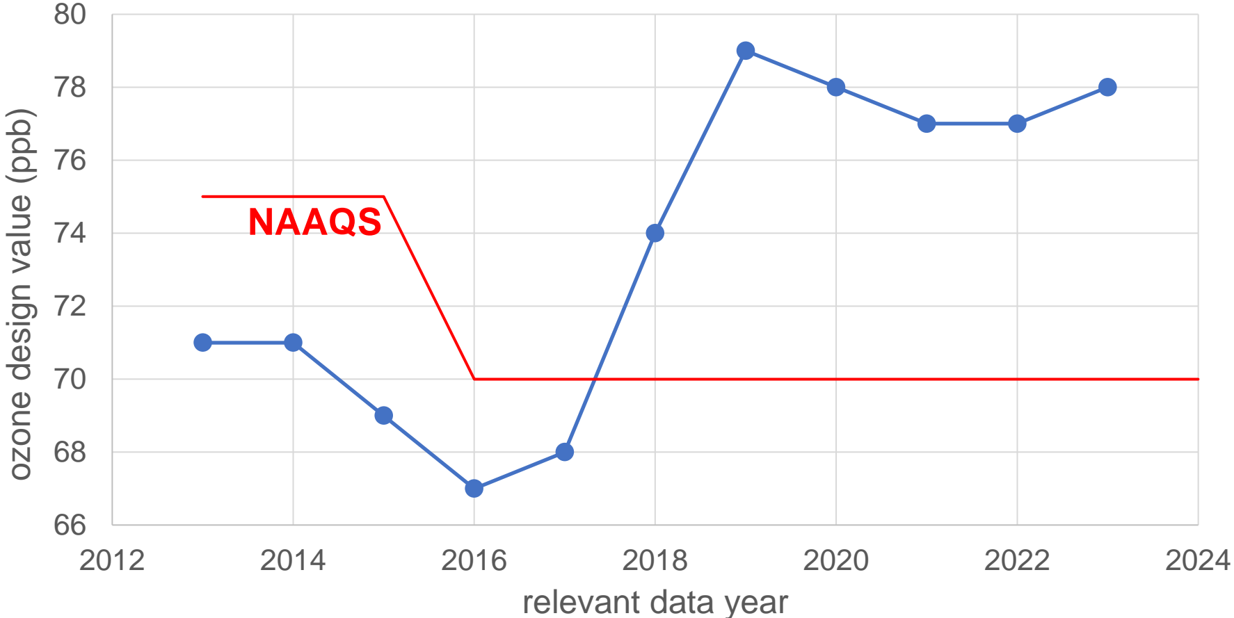
Ozone Design values, Eddy Cty (Carlsbad Caverns site)
